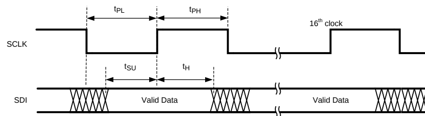
Figure 25. Write Timing
