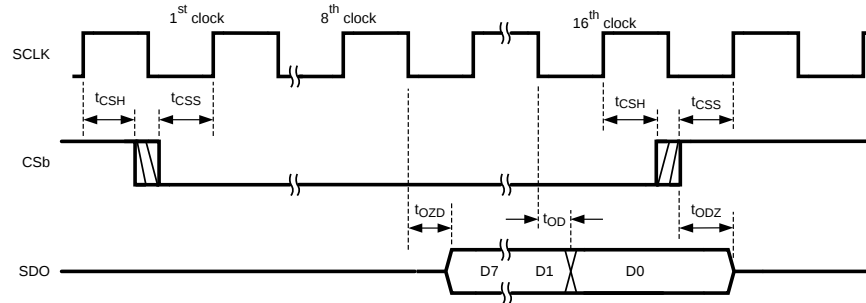
Figure 24. Read Timing
