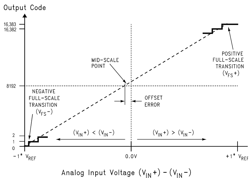
Figure 5. Transfer Characteristic
